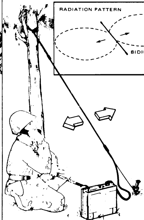
D. QUARTER-WAVE SLANT WIRE
